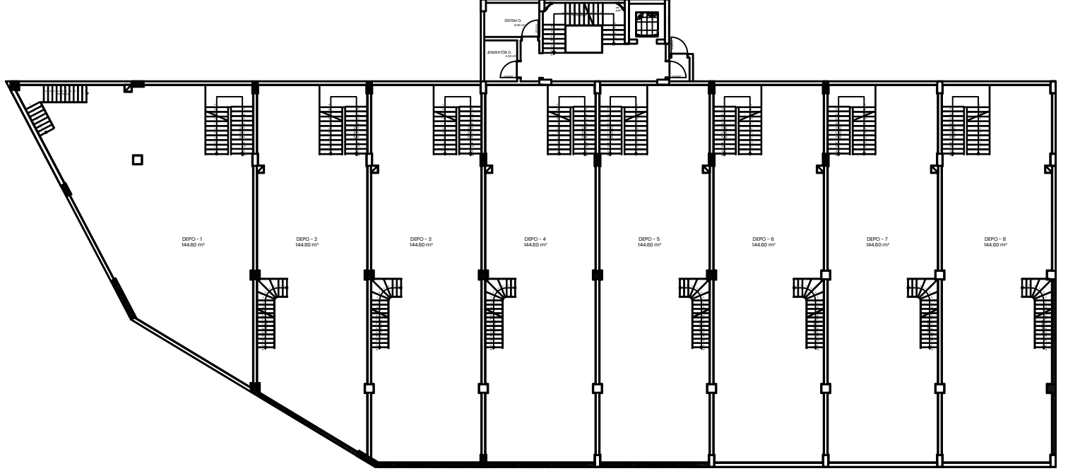
BODRUM KAT PLANI
